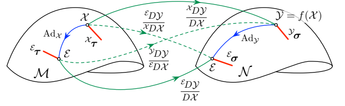
Figure 9. Linear maps between all tangent spaces involved in a function \mathcal{Y} = f(\mathcal{X}) , from \mathcal{M} to \mathcal{N} . The linear maps \varepsilon_{\tau} = \text{Ad}_{\mathcal{X}} x_{\tau} , \varepsilon_{\sigma} = \text{Ad}_{\mathcal{Y}} y_{\sigma} , \varepsilon_{\sigma} = \frac{\varepsilon_{D\mathcal{Y}}}{D\mathcal{X}} \varepsilon_{\tau} , and y_{\sigma} = \frac{{}^{\mathcal{X}} Df(\mathcal{X})}{D\mathcal{X}} x_{\tau} , form a loop (solid) that leads to (46). The crossed Jacobians (dashed) form more mapping loops leading to (47,48).
